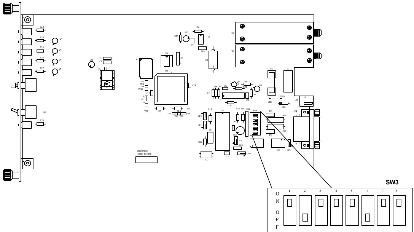
FIGURE 2. CIRCUIT DETAIL SHOWING SWITCH LOCATION
