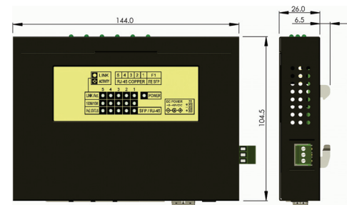
Dimensions (mm) with DRB-1 DIN Rail Mounting Kit
