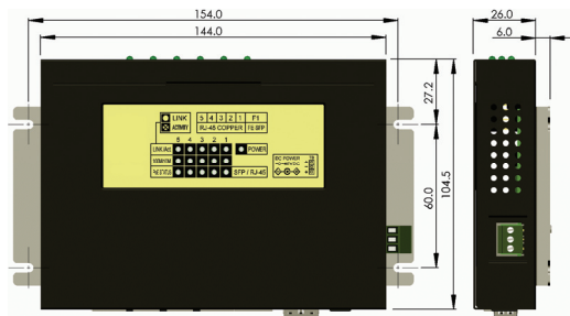
Dimensions (mm) with PMB-2 Panel Mount Kit
