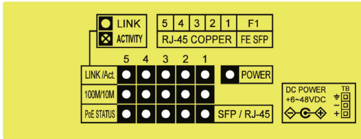
Top LED Status Label
